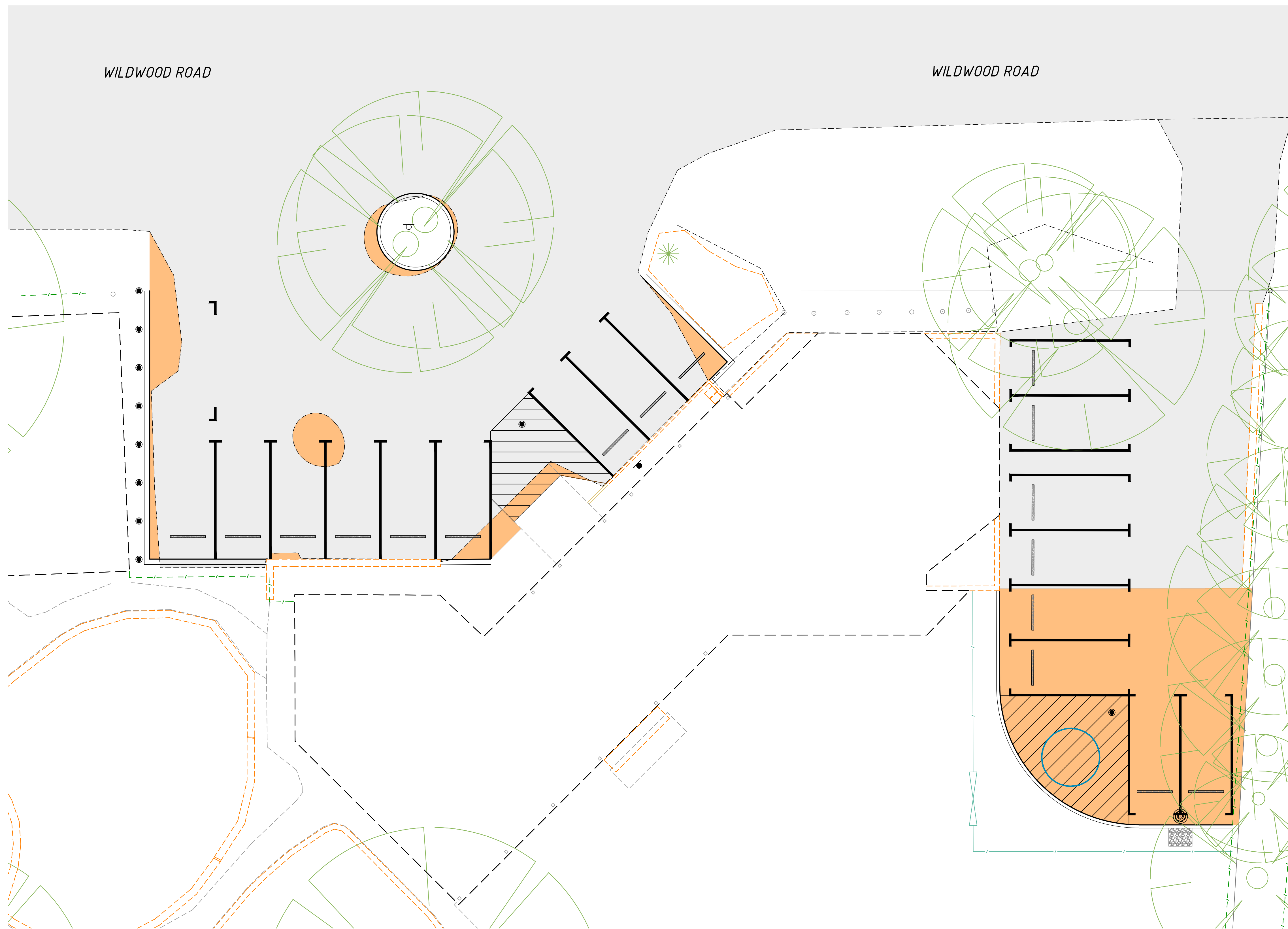
PLAN SCALE 1:100
